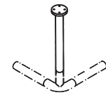
Deckenstütze Ceiling support 33.7100A ø 33 | 250-3999
