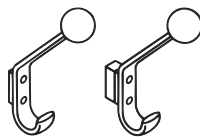
Garderobenhaken Coat hook 477.90.080 477.90.081 22 | 174 | 117 22 | 174 | 132
